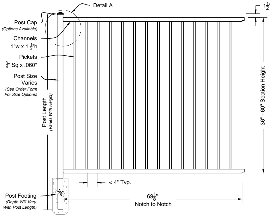
i 01 Alamo #400 6ft Fence Panel Shown As Commercial Series Scale: NTS
