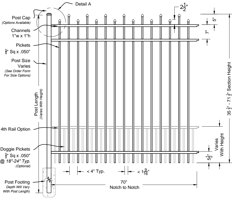
i 01 Californian #200 6ft Fence Panel Shown As Residential Series Scale: NTS
