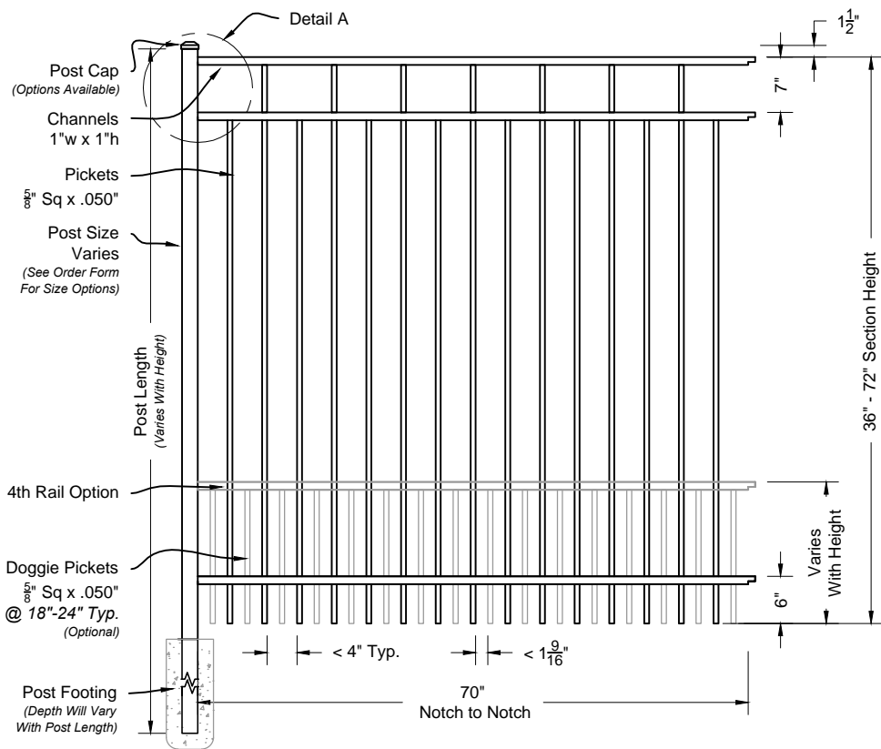
i 01 Carolina #403 6ft Fence Panel Shown As Residential Series Scale: NTS
