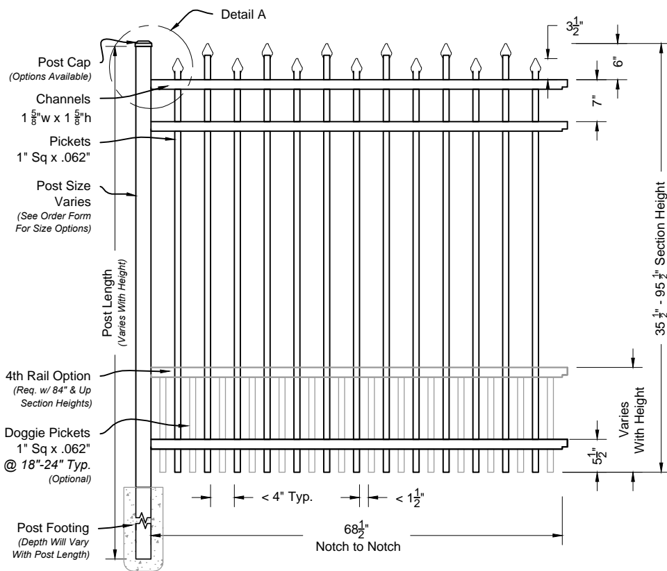
i 01 Californian #200 6ft Fence Panel Shown As Industrial Series Scale: NTS
