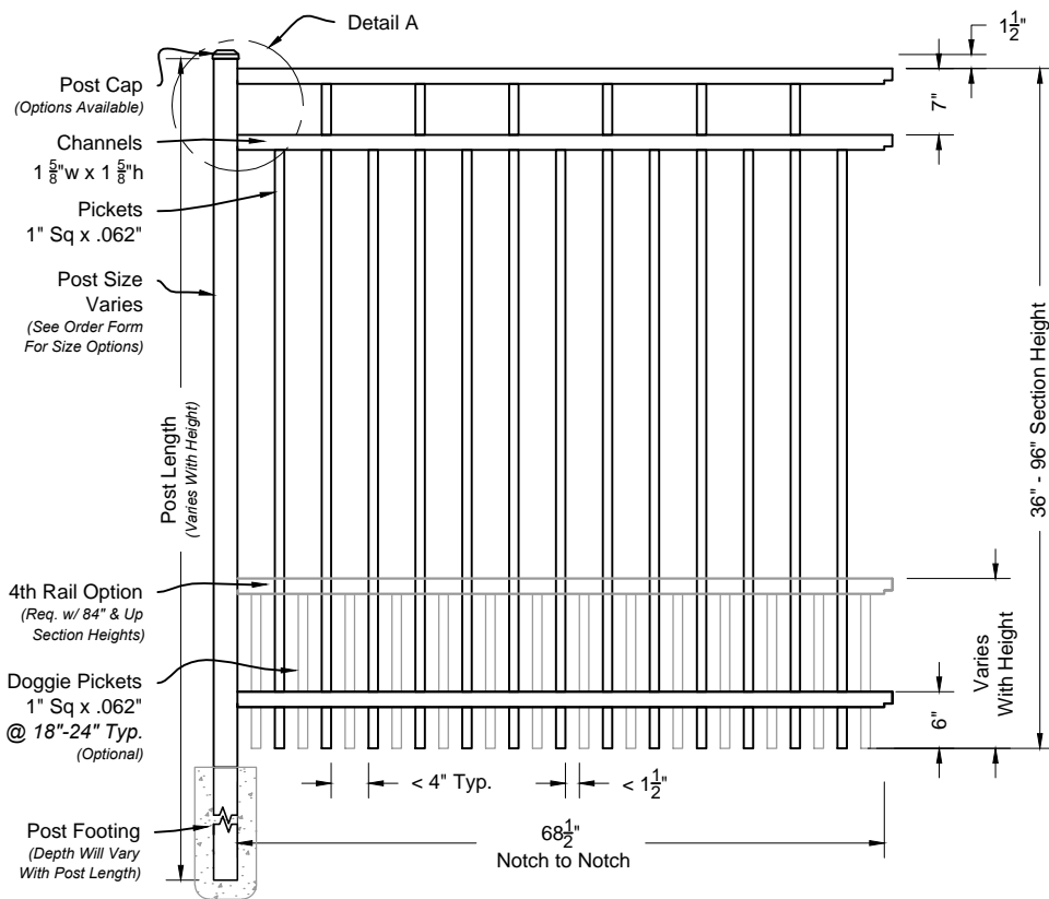
i 01 Carolina #403 6ft Fence Panel Shown As Industrial Series Scale: NTS
