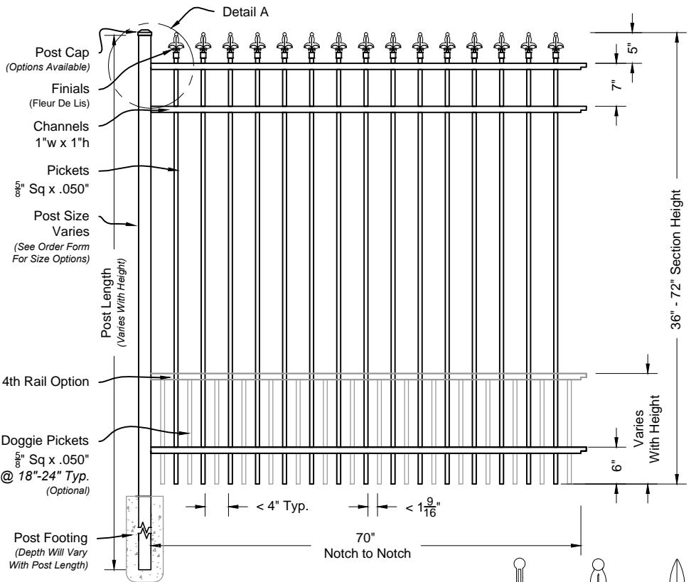
i 01 Finials #600 6ft Fence Panel Shown As Residential Series Scale: NTS
