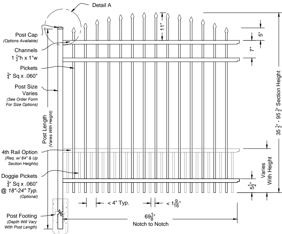
i 01 New Yorker #900 6ft Fence Panel Shown As Commercial Series Scale: NTS
