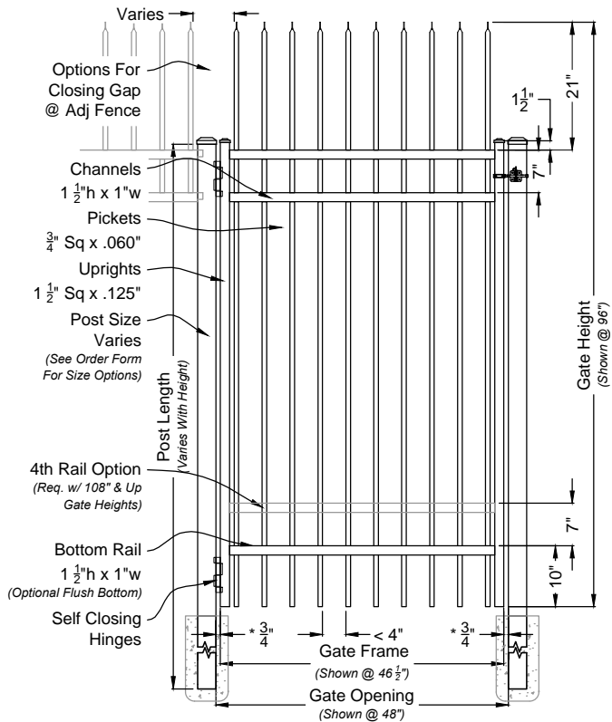
i 02 Talon Single Walk Gate #7000 Straight Rail Option Scale: NTS
