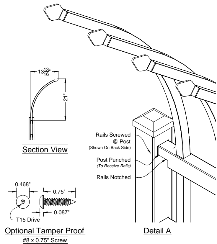
i 01 Talon #700 (Security) 6ft Fence Panel Shown As Commerical Series Scale: NTS
