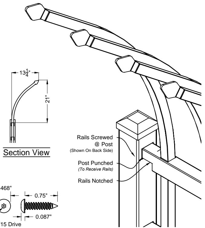
Optional Tamper Proof #8 x 0.75" Screw
