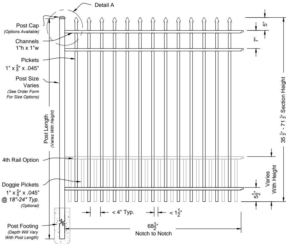
i 01 Maine #203 6ft Fence Panel Shown As Parkway Series Scale: NTS
