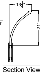
Samson 250N / 400N Adjustable Horizontal Gate Closer
