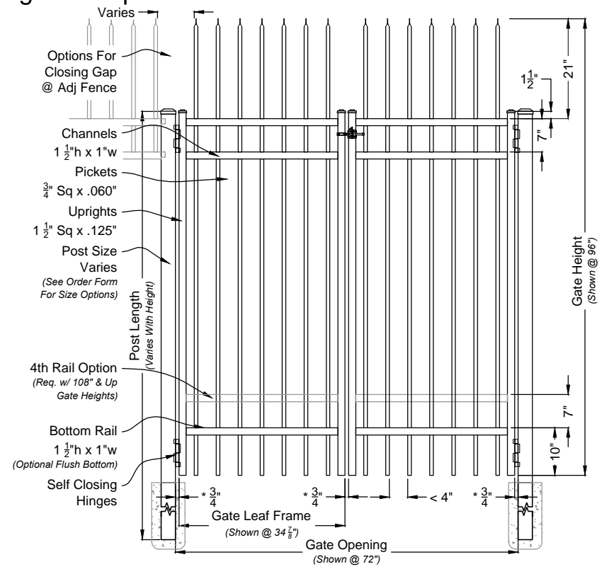
i 03 Talon Double Walk Gate #6700 Straight Rail Option Scale: NTS
