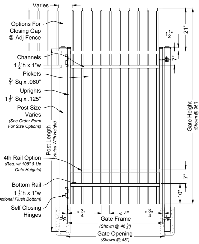
i 02 Talon Single Walk Gate #7000 Straight Rail Option Scale: NTS
