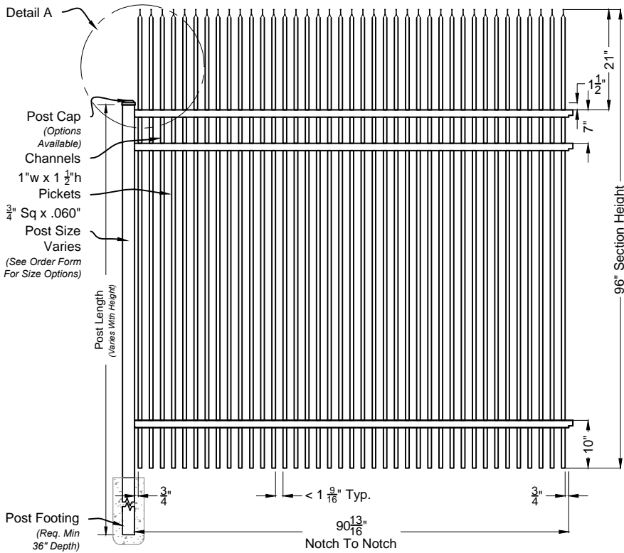
Talon #700 (Security) 8ft Fence Panel Shown As Commercial Series Scale: NTS
