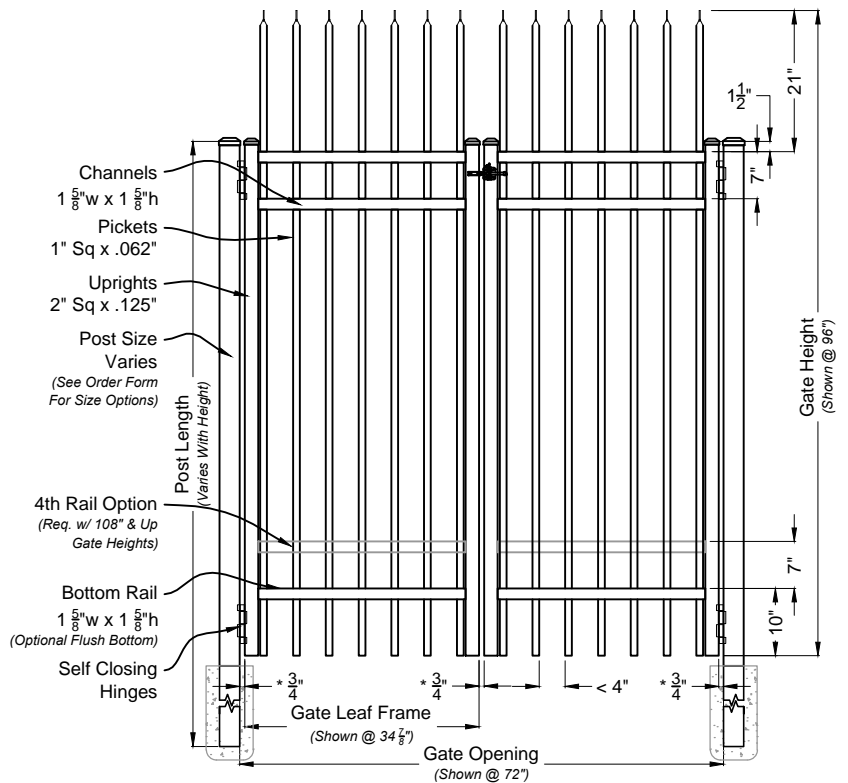
i Talon Double Walk Gate 03 #6700 Straight Rail Option Scale: NTS
