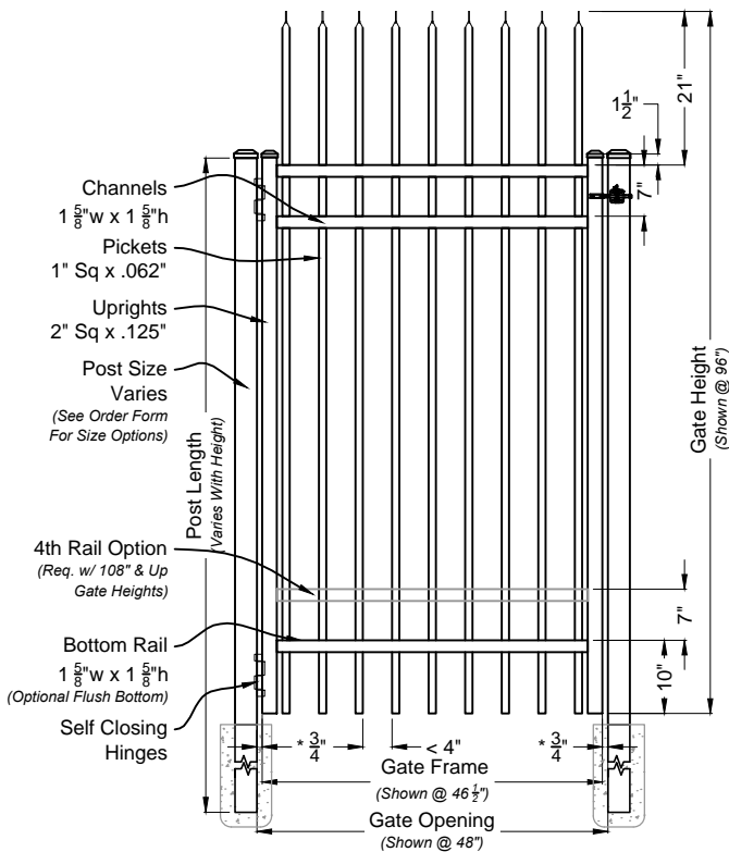
i Talon Single Walk Gate 02 #7000 Straight Rail Option Scale: NTS
