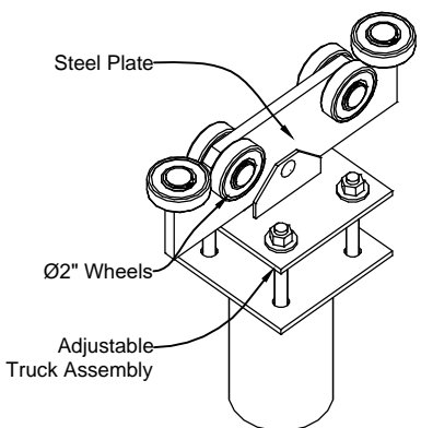
02 Truck Assembly Scale: NTS
