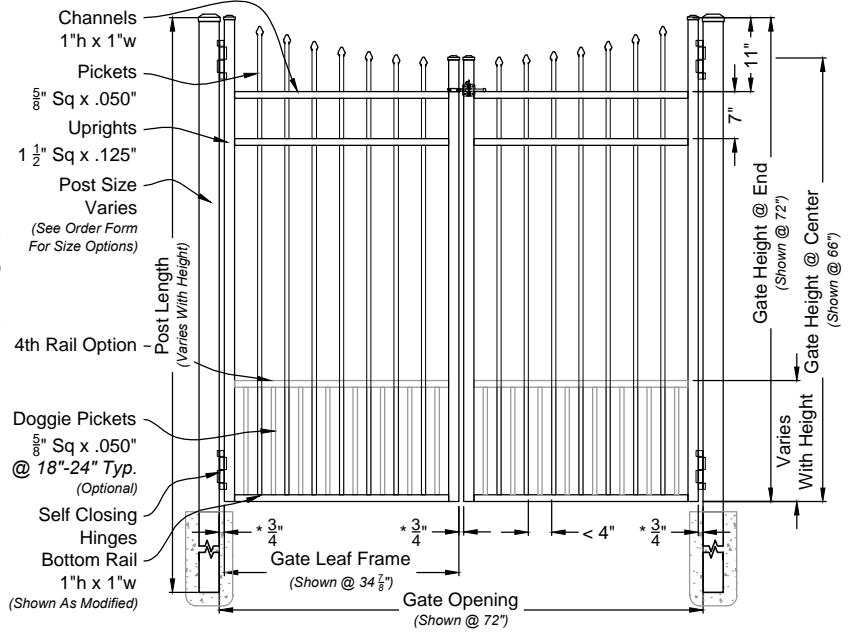
i 03 New Englander Double Walk Gate #6800M Straight Rail Option Scale: NTS
