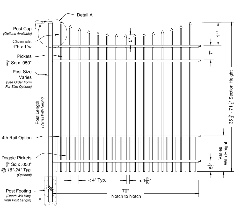
i 01 New Englander #800 6ft Fence Panel Shown As Select Residential Series Scale: NTS
