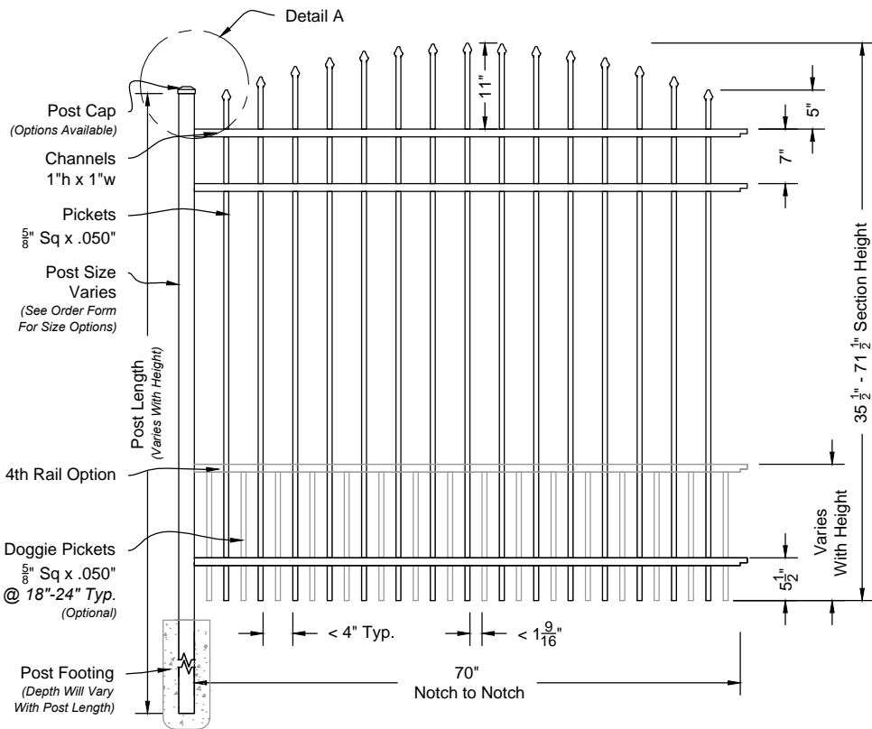
i 01 New Yorker #900 6ft Fence Panel Shown As Select Residential Series Scale: NTS
