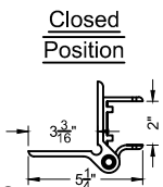
iDeal 180° Hinge Fits 4" Sq & Up Post Scale: NTS
